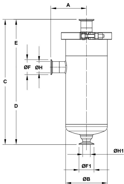
DIMENSIONS (mm)
