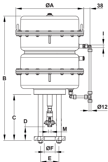
DIMENSIONS (mm)
